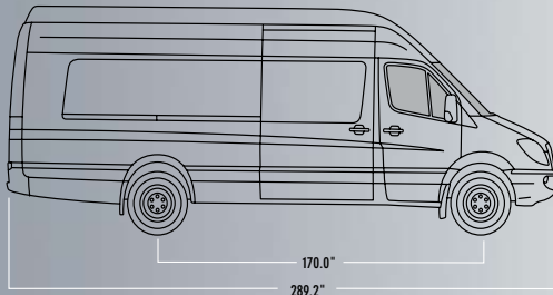
170" WHEELBASE EXTENDED
