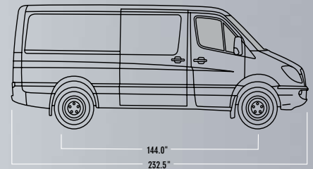
144" WHEELBASE
