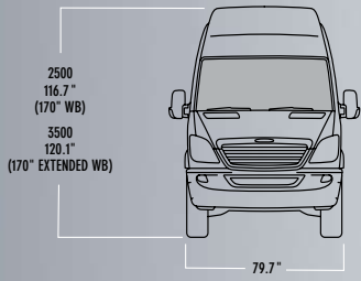
170" WHEELBASE EXTENDED
