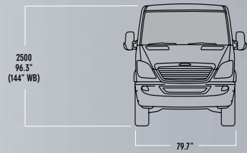
STANDARD ROOF
