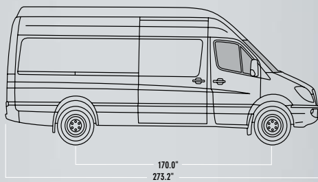
170" WHEELBASE
