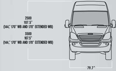
170" WHEELBASE
